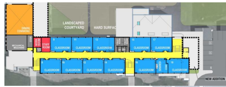
FIRST FLOOR PLAN - Diagram 'B-' SCALE: 1/8" = 1'-0" Lincoln Elementary School 1/21/2020
