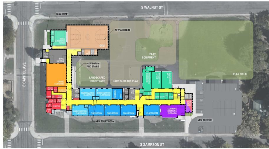
FIRST FLOOR PLAN - Diagram 'B-' SCALE: 1/8" = 1'-0" Lincoln Elementary School 1/21/2020
